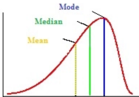
Left-Skewed (Negative Skewness)
