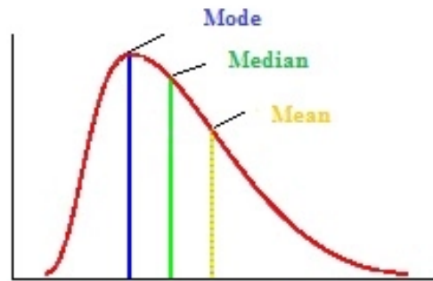
Right-Skewed (Positive Skewness)
